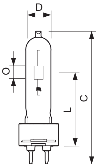
MASTERCcolour CDM-T 70W/830 G12 1CT
